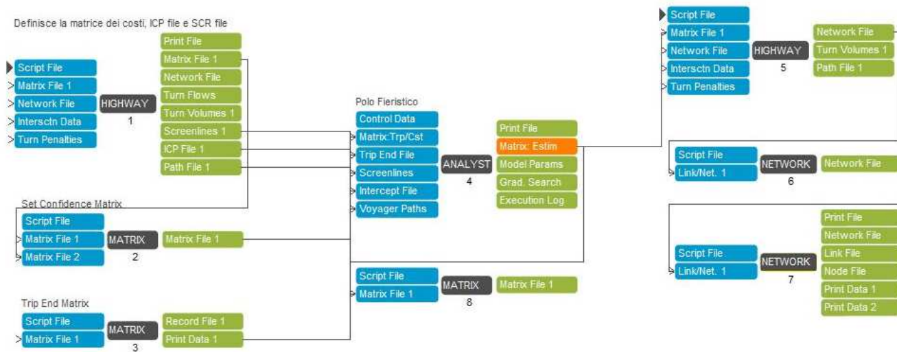
Figura 6-1: Application Manager modulo Matrix Estimation
