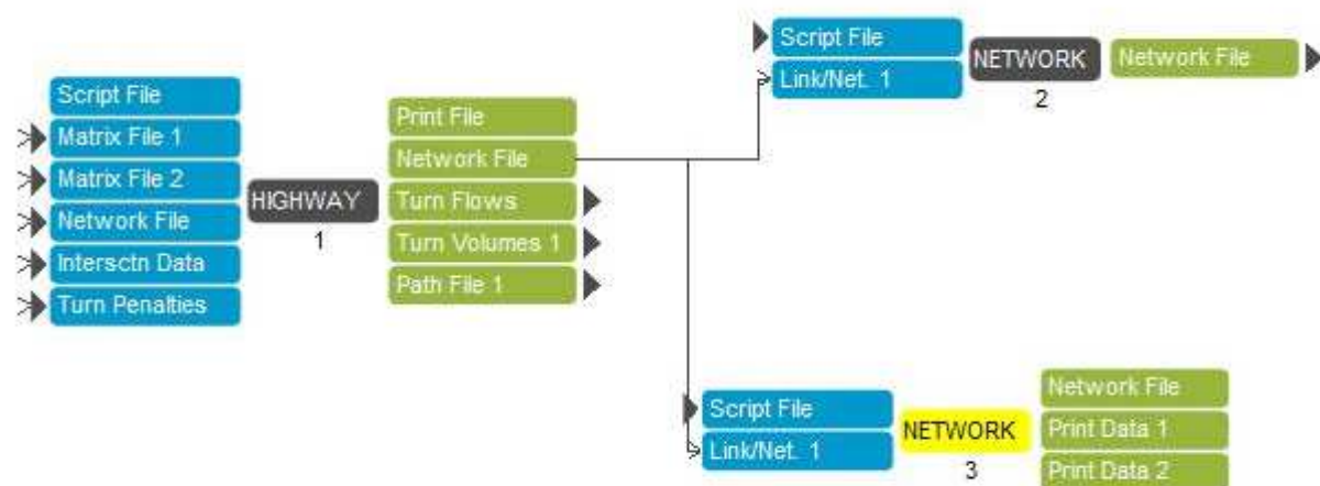
Figura 6-2: Application Manager modulo Highway di Cube
